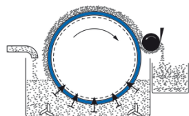
Roller discharge
